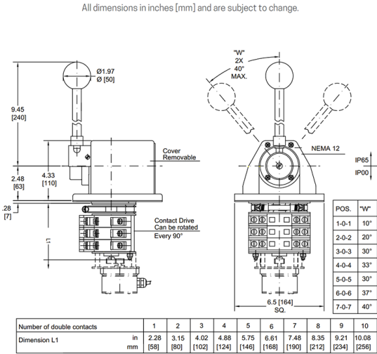
Overall dimensions. Shown with round ball handle.
