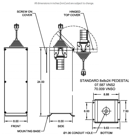
Standard 8 in x 8 in x 24 in pedestal for single axis VNSO and VNS2 joysticks
