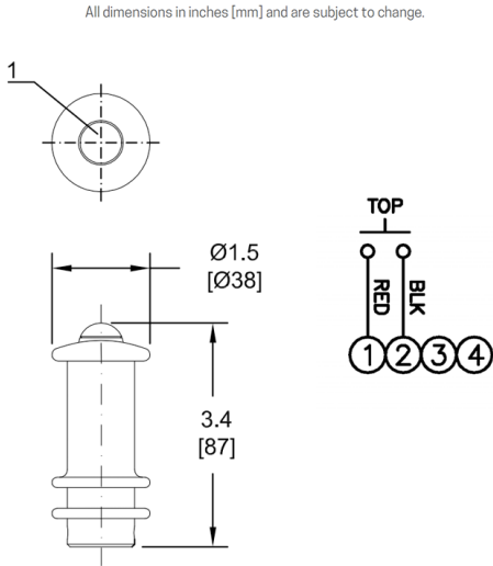
MG9 dimensions & wiring details
