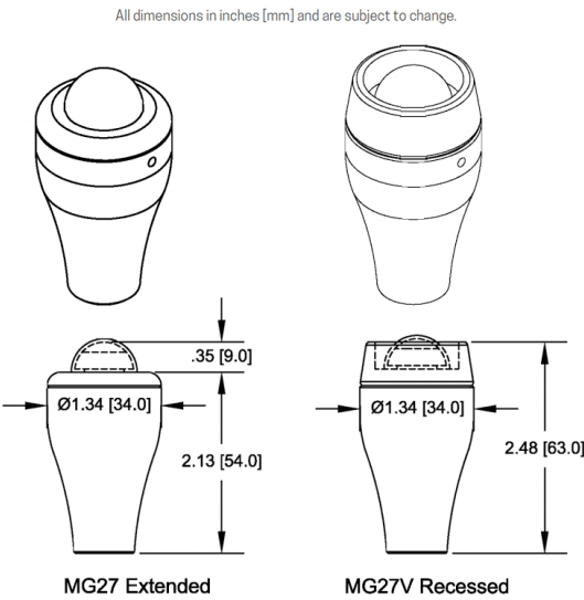
MG27 extended & recessed dimensions
