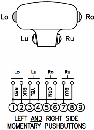
Left and ride side push button wiring details
