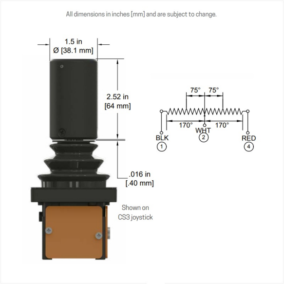
TH30 dimensions and wiring details
