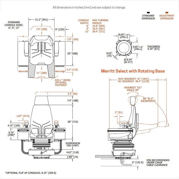
Rotating base model dimensions
