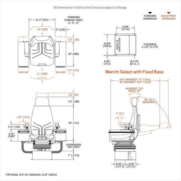
Fixed base model dimensions
