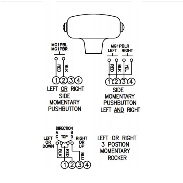
MG1 button and rocker switch wiring details
