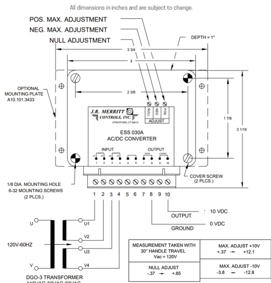
ESS 03A dimensions and wiring details
