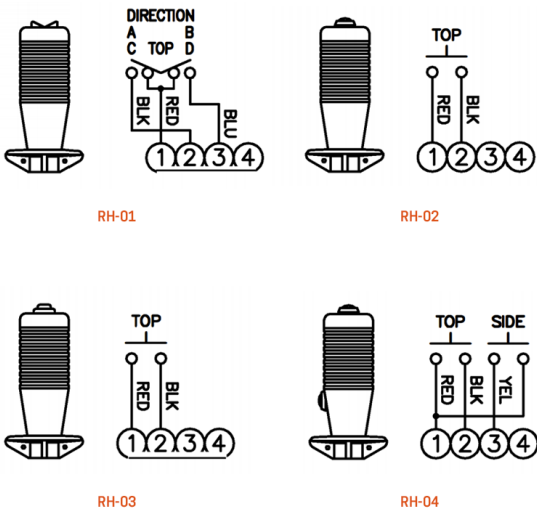
RH-01, RH-02, RH-03, RH-04 wiring details
