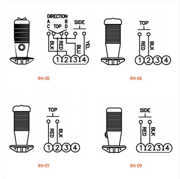
RH-05, RH-06, RH-07, RH-09 wiring details
