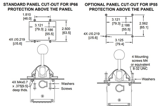
Standard and optional mounting details.
