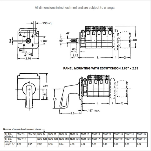
NSO-1 overall dimensions
